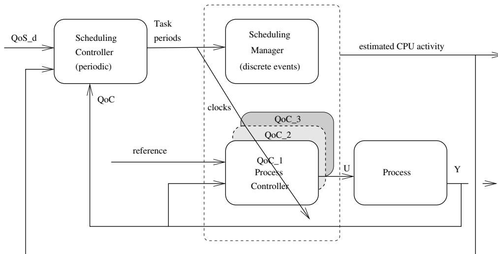
Figure 2. Hierarchical control structure.
