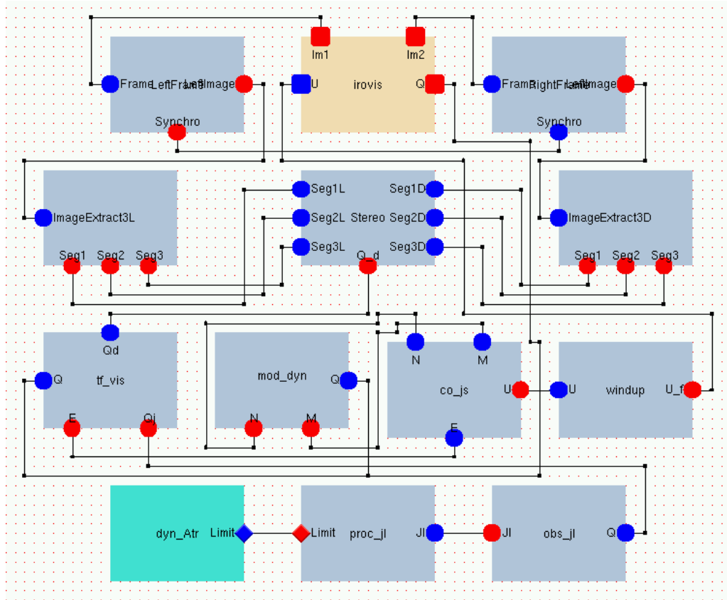
Figure 1. Orccad's GUI for control design.
