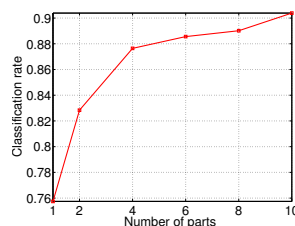
Figure 15. Classification results for the butterflies. (a) The second column shows the size of the model (top 10 parts) for each class (the sum of sizes of individual parts), and the size of the smallest and the largest parts are listed in parentheses. (b) Classification rate versus number of parts.
