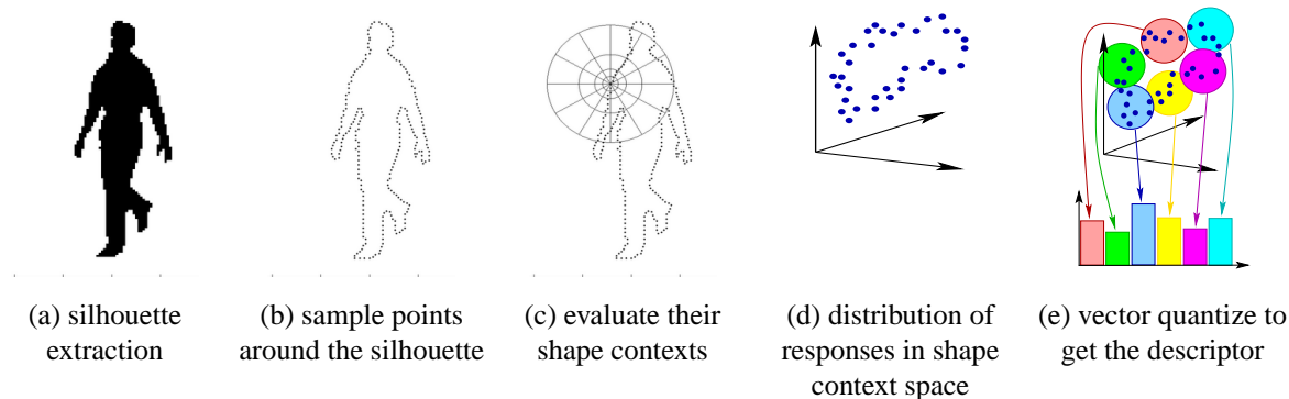
Figure 27. The extraction process for our robust descriptors of silhouette geometry. “Shape context” descriptors are evaluated at regular points around the silhouette, and the distribution of responses in shape context space is vector quantized into 100 bins to produce the final descriptor.
