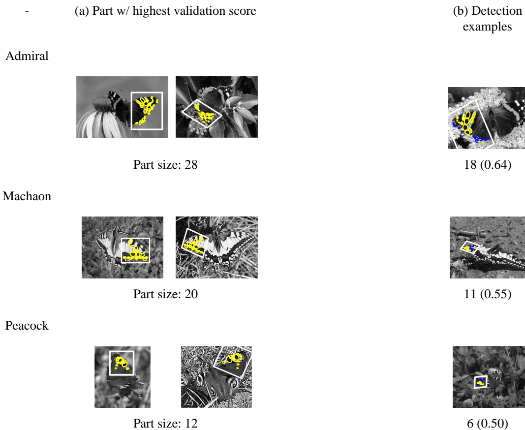
Figure 14. Butterfly modeling and detection examples. (a) The part with the highest validation score for a class. The part size is listed below each modeling pair. (b) Example of detecting the part from (a) in a single test image. Detected regions are shown in yellow and occluded ones are reprojected from the model in blue. The total number of detected regions (absolute repeatability) and the corresponding repeatability ratio are shown below each image.
