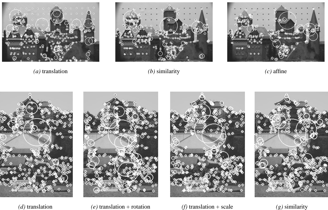
Figure 3. Some examples of keypoints found by our detectors. The detectors have selected points that have maximal local stability under the indicated transformations. For example, the dots in the background of the top image provide good stability against translations but poor stability against rotations, so they are selected as keypoints under the translation group, but not under the group of similarity transformations.
