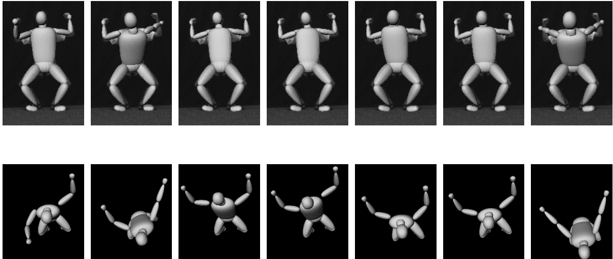
Figure 25. Some examples of ‘reflective’ local minima induced by the kinematic structure of the problem of motion capture from monocular images. The minima were found by eigenvector tracking, one of our Newton based search methods for nearby local minimum. The images show the human model from the original camera viewpoint and from a synthetic overhead viewpoint. Note the pronounced forwards-backwards character of these reflective minima, and the fact that in each case the model fits the original image well.
