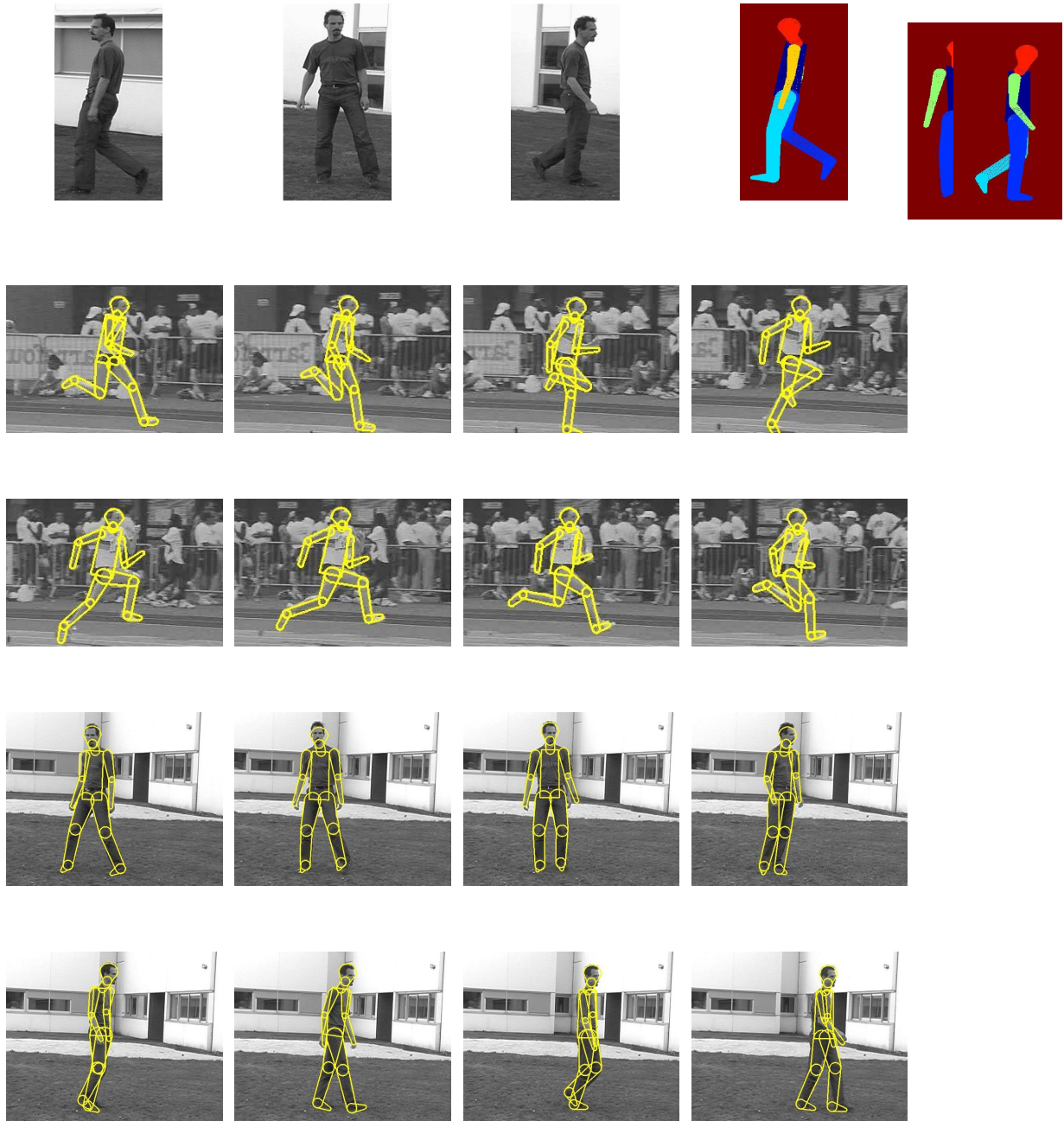
Figure 26. Some examples of 2D human tracking with our learned dynamical model. First row: In preparation for learning, the configuration of the model is marked by hand in each training image. Here we show three images with their corresponding configurations and visibility maps. Rows 2–3: Tracking a running athlete. The model was learned on another athlete but follows this one well except that the left arm was not correctly initialized because it was invisible in the initial image. Last 2 rows: Tracking a turning movement through changes of model aspect from face to side view.
