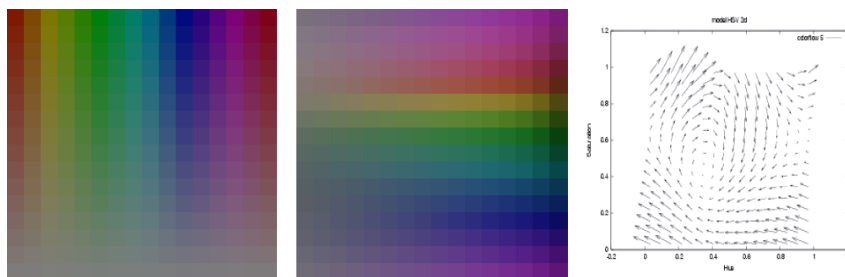
Figure 6. An illustration of the color flow model. Left : the reference color map (Hue / Saturation representation). Middle : the color map for a new illumination of the scene. Right : the transformation between the two maps (vectors represent individual color changes).
