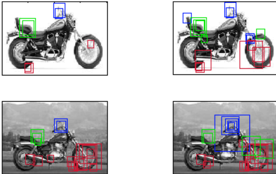
Figure 7. Recognition of motorbike parts using HDDA (left) and SVM (right). The colors blue, red and green are respectively associated with the handlebar, wheel and seat features.
