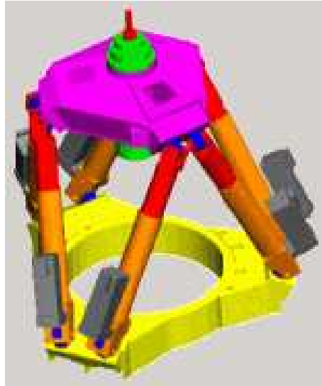
Figure 1. An Hexapod
