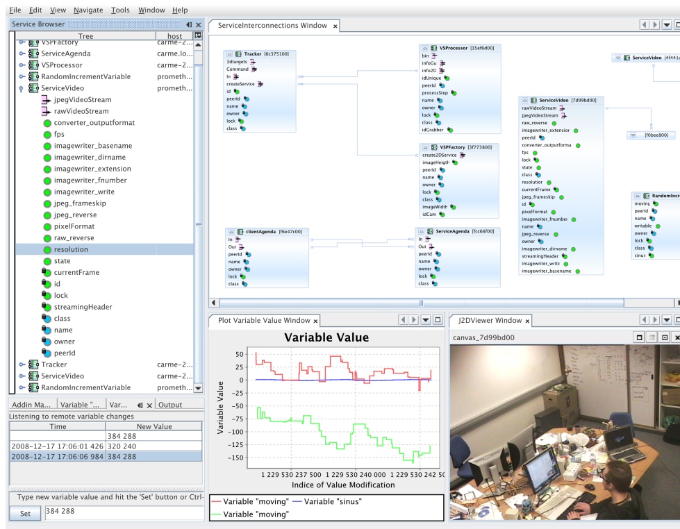
Figure 6. OMiSCID GUI showing a list of running services and some modules for service interconnections, variable plotting, live video stream display and variable control
