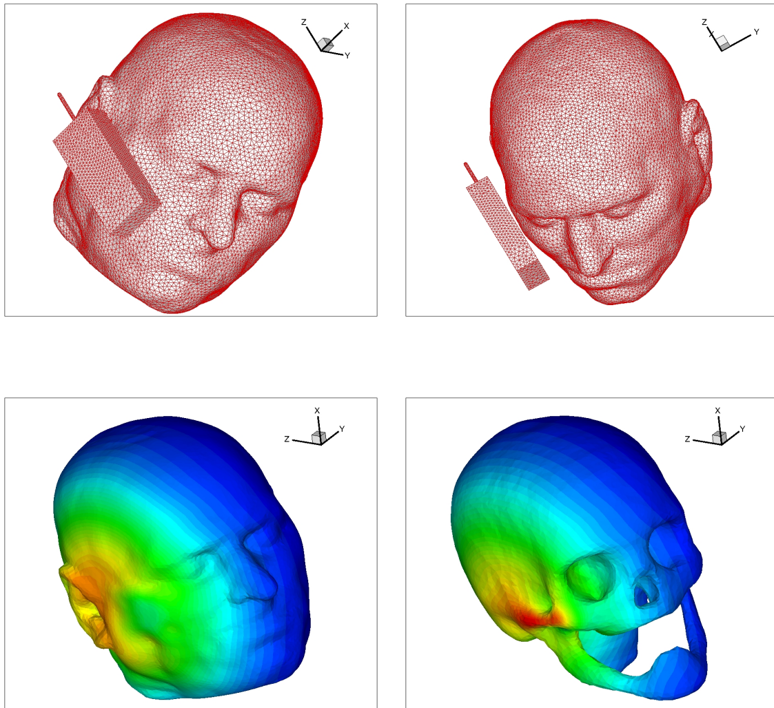
Figure 1. Exposure of head tissues to an electromagnetic wave emitted by a localized source Top figures: surface triangulations of the skin and the skull. Bottom figures: contour lines of the amplitude of the electric field.
