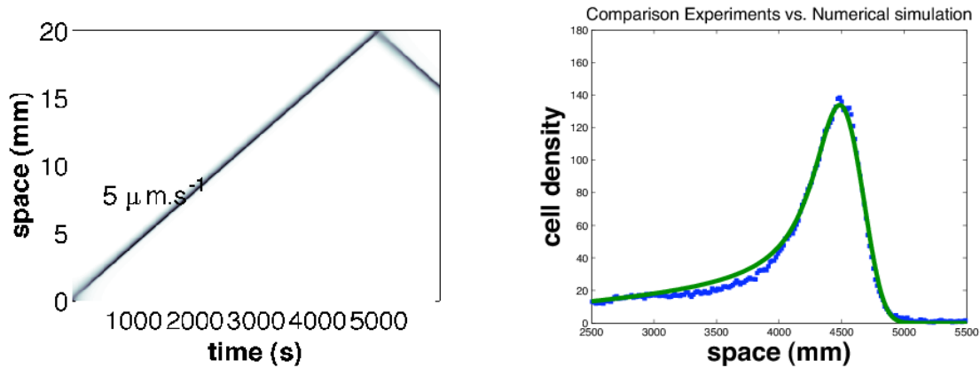
Figure 2. (left) Numerical simulation of a traveling pulse obtained with the kinetic model (right) Comparison between the bacteria density measured experimentally (blue dots) and the density computed from the kinetic model.
