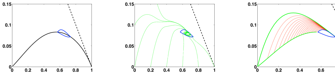
Figure 4. Dynamics of trajectories of the control system projected on the simplex. (left) Remarkable sets in the simplex: the line of eigenvectors parametrized by the control parameter, and the small "ergodic" set. (middle) All trajectories eventually enter the ergodic set. (right) We prove a tunnelling effect: all trajectories are confined in a neighbourhood of the ergodic set, and moves towards it.
