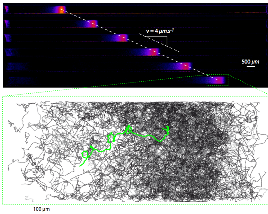
Figure 1. Bacterial waves traveling in a narrow channel (experiments) (Figure from the PhD thesis of J. Saragosti, Institut Curie 2010).
