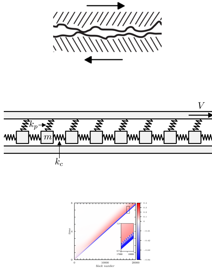
Frictional interface and solitary waves in the Burridge-Knopoff model [80]
