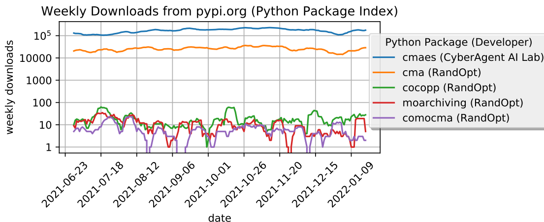
Figure 1: Weekly downloads from PyPI of RandOpt related Python software packages.
