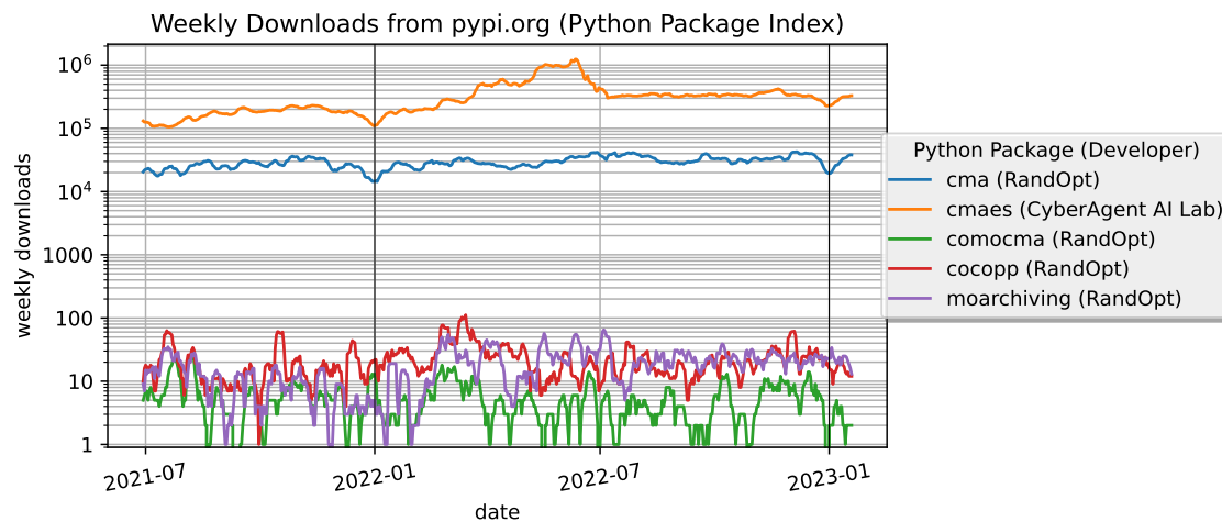
Figure 1: Weekly downloads from PyPI of RandOpt related Python software packages since mid 2021.
